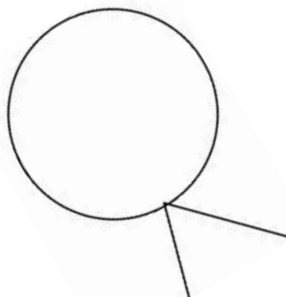
Figure 9. Non-circumferential angles
