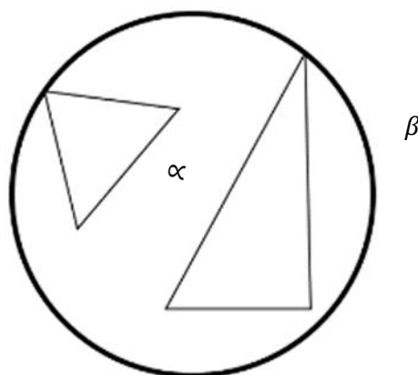
Figure 3. Strings and lines \alpha \neq \beta
