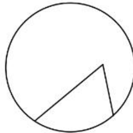
Figure 7. Non circumferential angles
