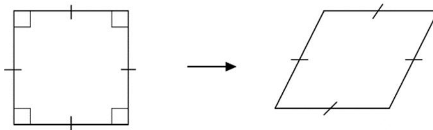
Figure 1. The square of the parallelogram family
