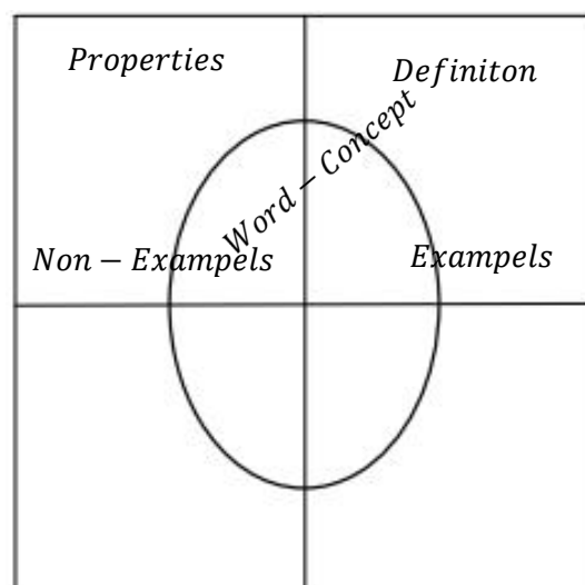
Figure 5. Frayer model
