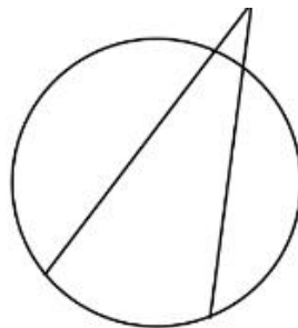
Figure 8. Non-circumferential angles
