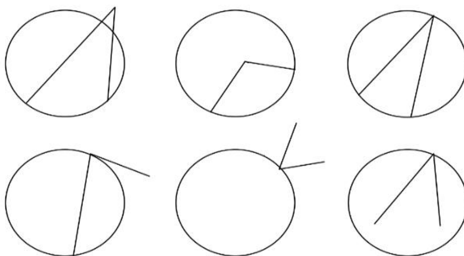
Figure 10. Which can be a circumferential angle?
