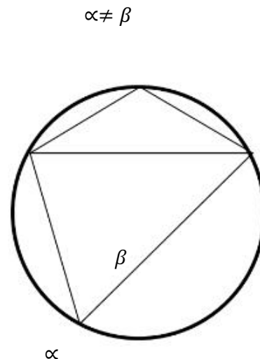
Figure 4. Circumferential angles on the same side
