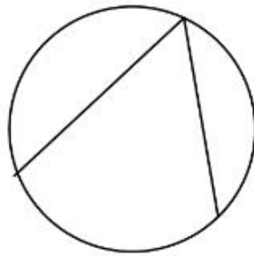
Figure 6. Circumferential angles
